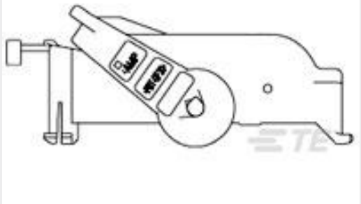
TE 产品编号1473247-1 MQS 81P LEVER(R) ASSY
