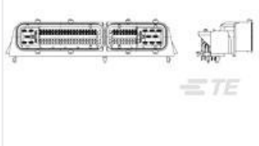
TE 产品编号1241434-1 121pos hybrid MQS .63 header 90deg
