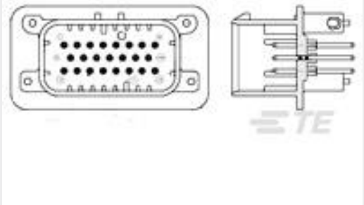
TE 产品编号1-776228-5 HEADER ASSY, 23 POS VERTICAL
