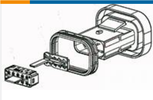
TE 产品编号1801610-1 BULK HEAD, MCON, 10W, CLIPPED
