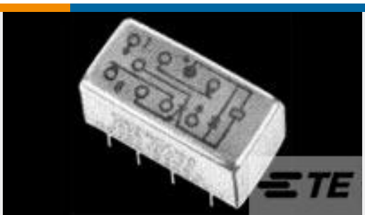
TE 产品编号3-1617073-8 3SBC2096A2 = M39016/37-026P
