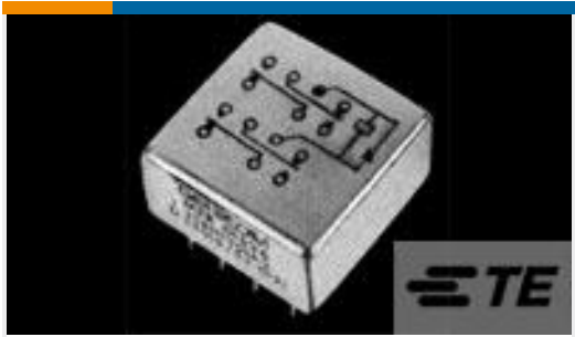
TE 产品编号3-1617076-0 3SBH1261A2 = M39016/54-011M
