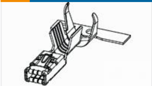
TE 产品编号1670804-3 MCON 2.8 TERMINAL - LL
