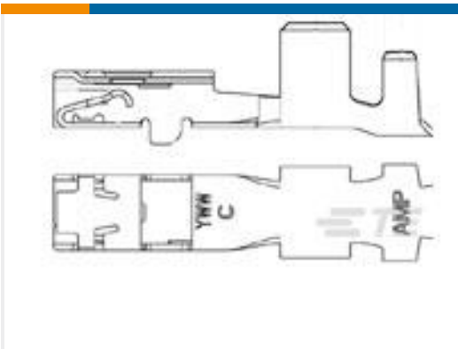
TE 产品编号1326030-5 2.8MM RECP,UNSEAL,22AWG,REVREE
