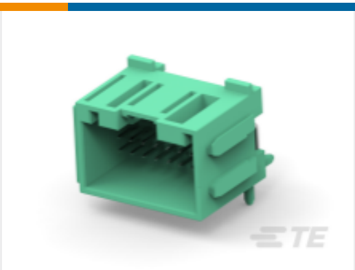
TE 产品编号2311622-3 16POS,TAB0.63X0.63,HDR ASSY, 90DEG,SLDR
