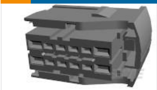
TE 产品编号284853-2 12 POS FEMALE CONNECTOR ASS'Y
