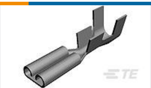
TE 产品编号42021 FASTON 250 (6.3MM) REC 16-12 AWG TPBR
