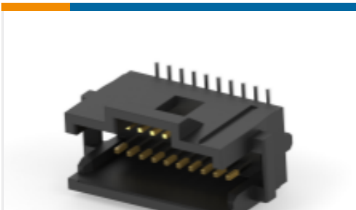
TE 产品编号2-1825601-0 20 SYS50 SMT HDR DR SHD W/O CAP
