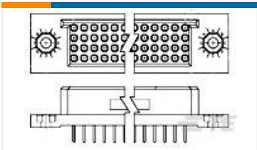
TE 产品编号5-533285-6 BOX II 4 ROW RECP ASSY 180 POS
