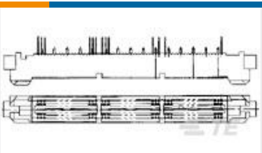
TE 产品编号5767082-1 MICT,495,PLUG,038,PDNI,BARBLES
