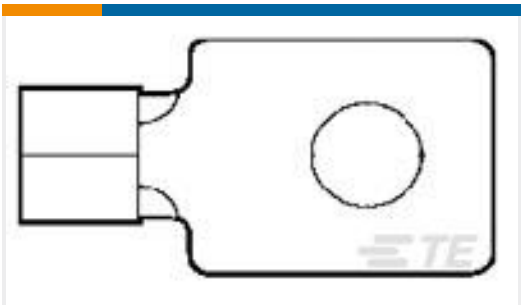
TE 产品编号34263 SOLIS RECT 22-16COMM22-18MIL 6
