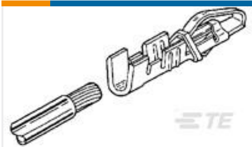
TE 产品编号280623-2 AMP LEAF CTC 22-18 AWG
