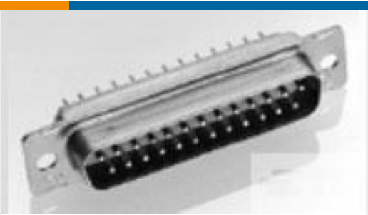
TE 产品编号1757819-1 AMPLIMITE,ASY,PLUG,STD,109,ZN,1
