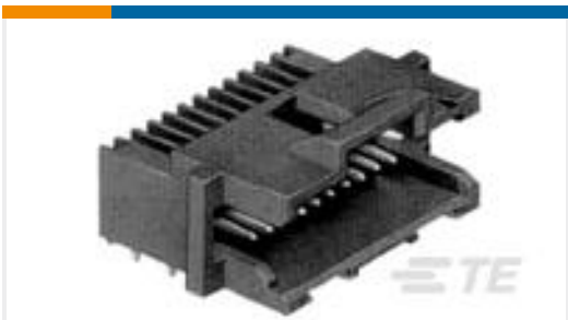
TE 产品编号104069-4 10 SYSTEM 50 HDR DRRA SHRD
