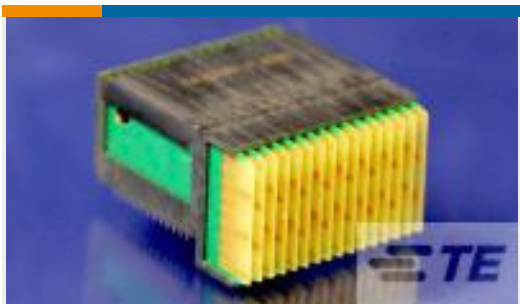
TE 产品编号1410970-3 MULTIGIG RT T2 7RW RTM MIXED DC
