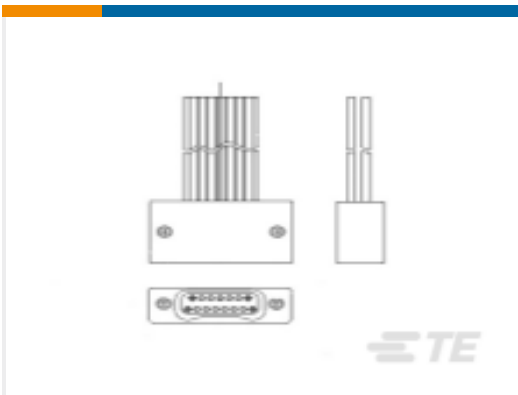
TE 产品编号1589477-4 STM025SC2DC012N = WDUALOBE
