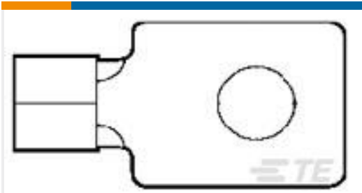
TE 产品编号35129 TERMINAL,BUDG RECT 16-14 .110
