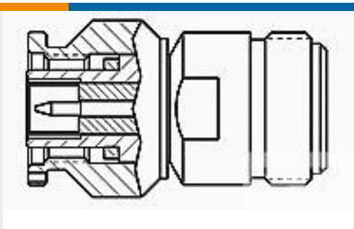
TE 产品编号1484244-1 ADAPTER, TNC PLUG TO N JACK 3682 2311 02
