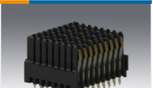
TE 产品编号 1410186-2 MULTIGIG RT T2 .8" BP HALF LEFT
