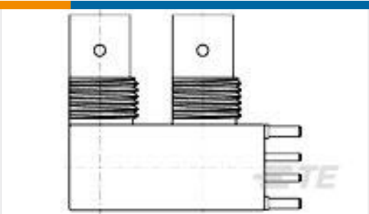
TE 产品编号1274663-2 JACK, 2 POSITION, STACKED R/A, MINI BNC
