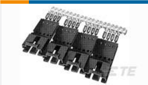
TE 产品编号103945-1 8X2 MTE SHRD PIN SR LATCH .100
