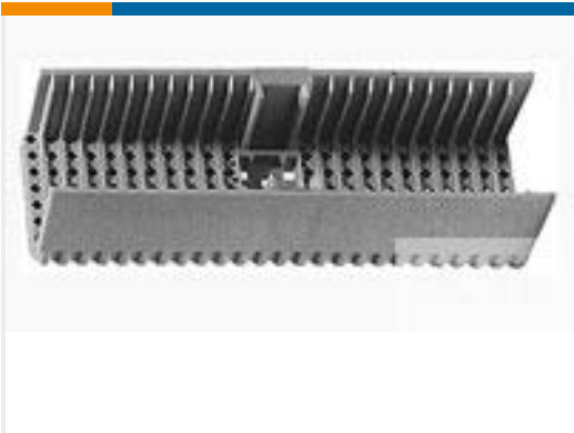
TE 产品编号646483-5 2MM H.M.,A/B 19 SHROUD 4.5MM
