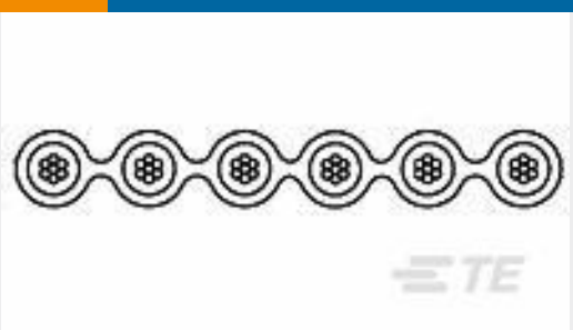
TE 产品编号2-162400-0 20P. RIBBCBL 28AWG P1.27 RL=100FT
