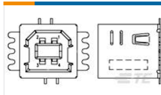
TE 产品编号1734517-1 STD USB TYPE B, VERTICAL, SMT, GRD FINGER
