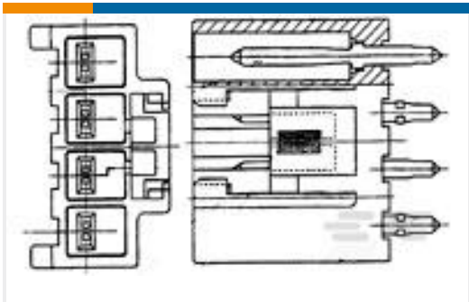
TE 产品编号1-178487-1 UP 3.96 4P TAB HDR NAT TYPE 2
