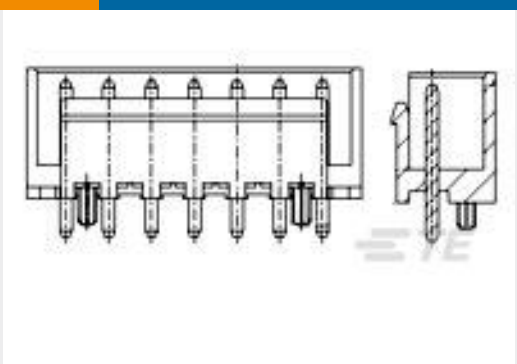
TE 产品编号1744357-5 3.96 EP SHROUDED HDR ASSY 2P W
