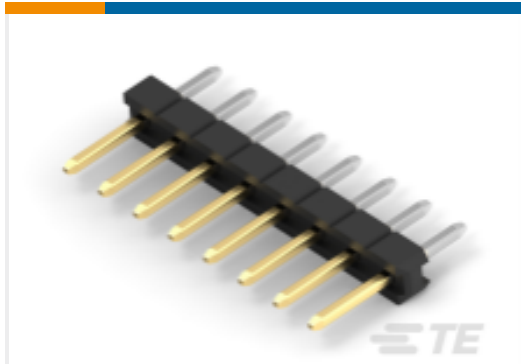
TE 产品编号1-2355177-0 10P,2MM,BRK HDR,SRVT,2.8,0.38AU, TB
