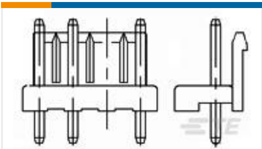
TE 产品编号172653-4 DRAWER CONN MALE HSG ASSY 24P
