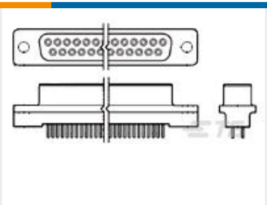
TE 产品编号745078-4 25 RCPT SP/AP SCRLK
