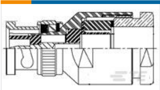
TE 产品编号1337771-4 50 OHM COAX BNC STR PLUG STR P
