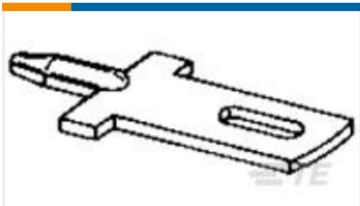
TE 产品编号735084-2 FASTON .110 (2.8 MM) .0198 X.550 TPBR
