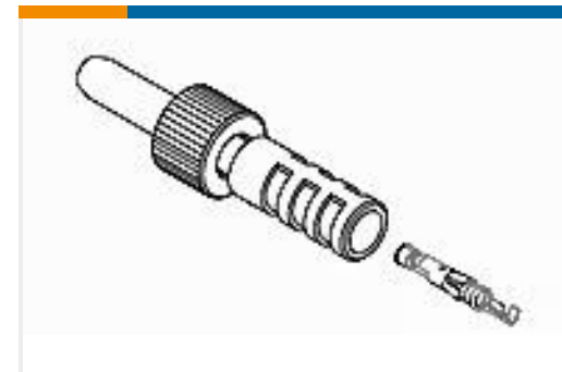
TE 产品编号861610-5 LGH, HIGH VOLTAGE PLUG
