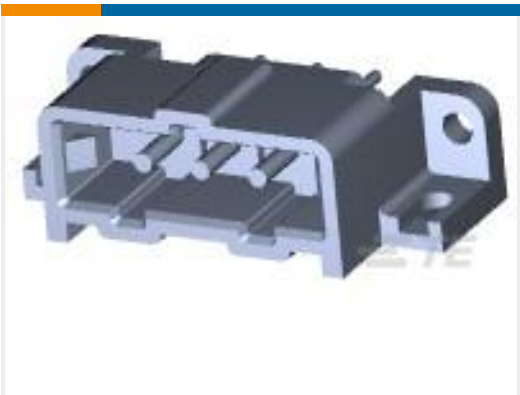
TE 产品编号207365-7 METRIMATE PIN HEADER ASSY,3P
