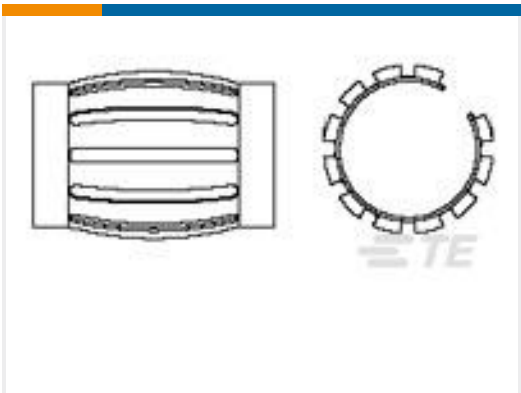
TE 产品编号1-192048-1 LA6 .127, .004, GOLD PL
