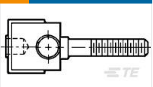
TE 产品编号532924-3 HDI POWER CONTACT ASSY
