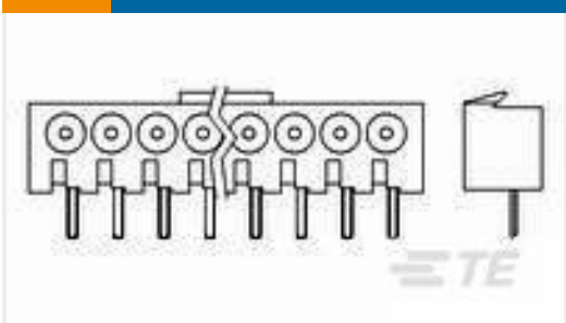
TE 产品编号1888290-5 .100 SRRA T-H, Latchg Flexstrip Recep
