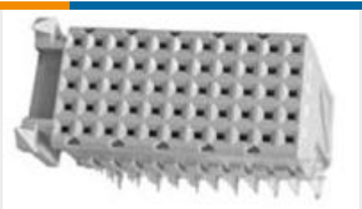
TE 产品编号100161-1 Z-PACK/C F-HDR 55P
