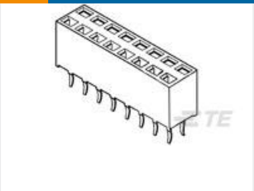
TE 产品编号1-215307-7 2X17P HV100 REC CON. TE, 7.0MM
