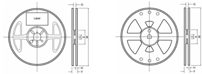
7" Reel (M)
