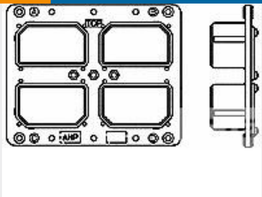
TE 产品编号1218231-1 M4P106P106P106P-2300(200)
