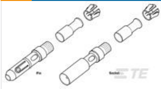
TE 产品编号201145-4 COAX MINIATURE SOCKET ASSY
