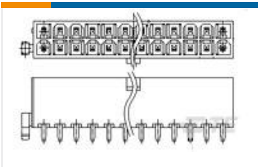
TE 产品编号1775099-8 ATX PWR CONN 1 BDLK 12 POS
