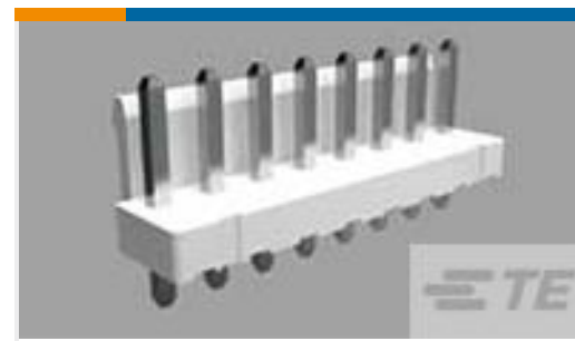
TE 产品编号1744037-2 02P EC PWR.200 CL HDR ASSY VRT
