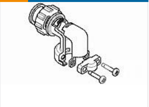
TE 产品编号1546350-2 R/A CABLE CLAMP KIT, SZ 23, CPC
