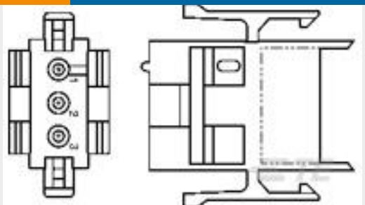
TE 产品编号1-640508-0 03P MR II CAP HSG V0 RED
