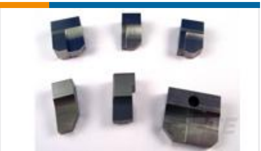
TE 产品编号1803040-2 COMBINATION ANVIL, BENDING
