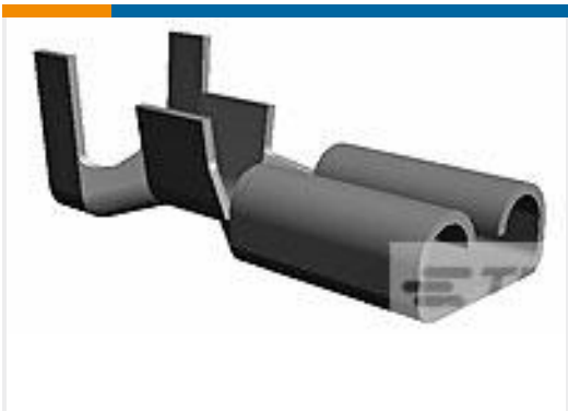
TE 产品编号170467-1 187 FASTON, REC., 18-14 AWG, TPPB
