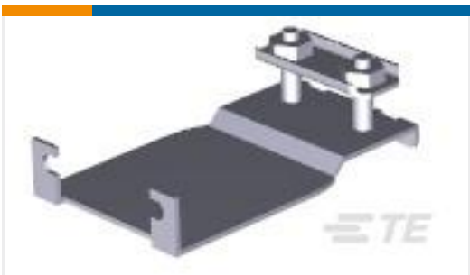
TE 产品编号201843-1 STRAIN RELIEF CLAMP (14) POS.
