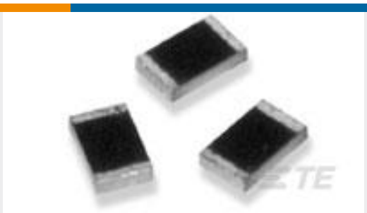
TE 产品编号1879269-1 RP 2A 22R1 0.1% 15PPM CUT LENGTH
