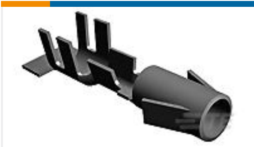
TE 产品编号925866-2 .140 DIA SOCKET
