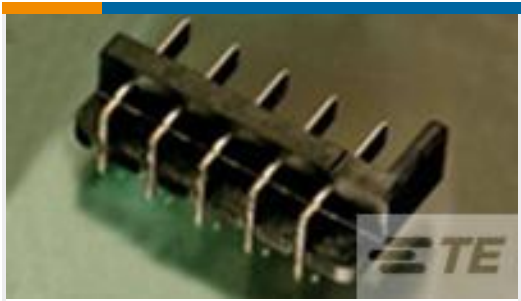
TE 产品编号5787246-1 HDR ASY,RA,LKEY,STR TAIL,10.8V
