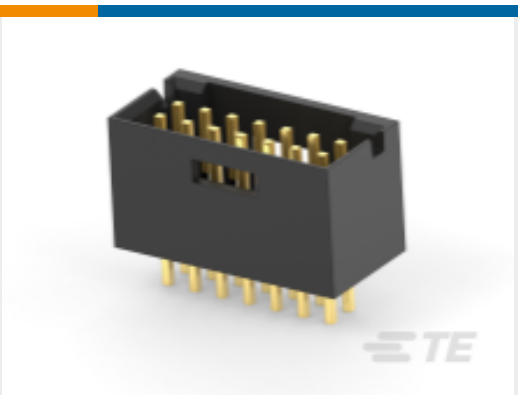
TE 产品编号87690-3 14 MODII HDR DRST SHRD .100CL
