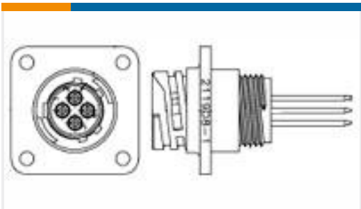
TE 产品编号1-788130-1 CPC RCPT,PSTD,SZ 11-4 LF
