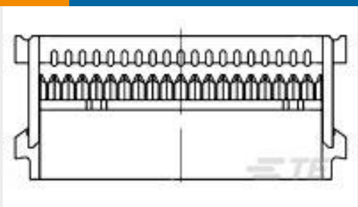
TE 产品编号1-1658526-6 609-2641LF FEM SOCKET,LEAD FREE
